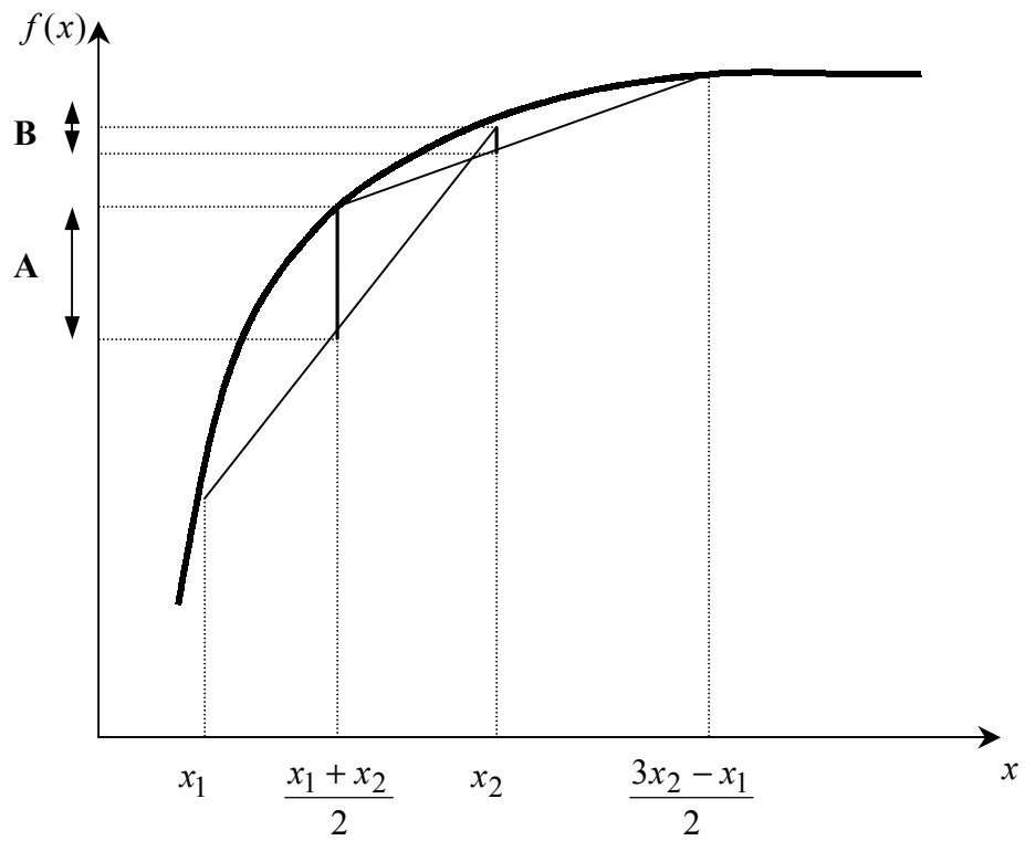
Figure 1: Illustration of 3-convexity
